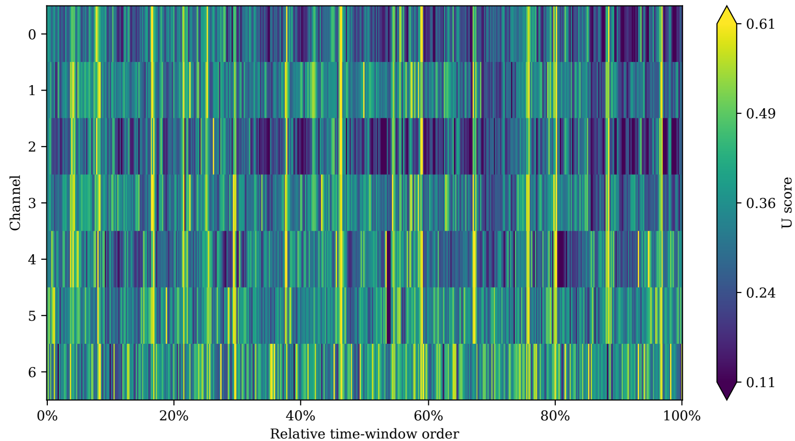
ETTh1: U across channels and time windows
