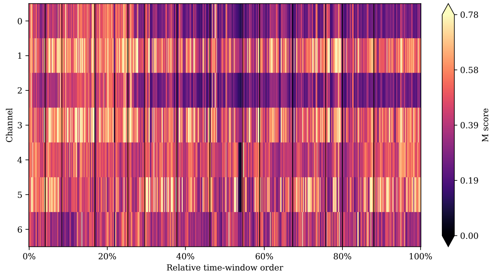
ETTm1: M across channels and time windows
