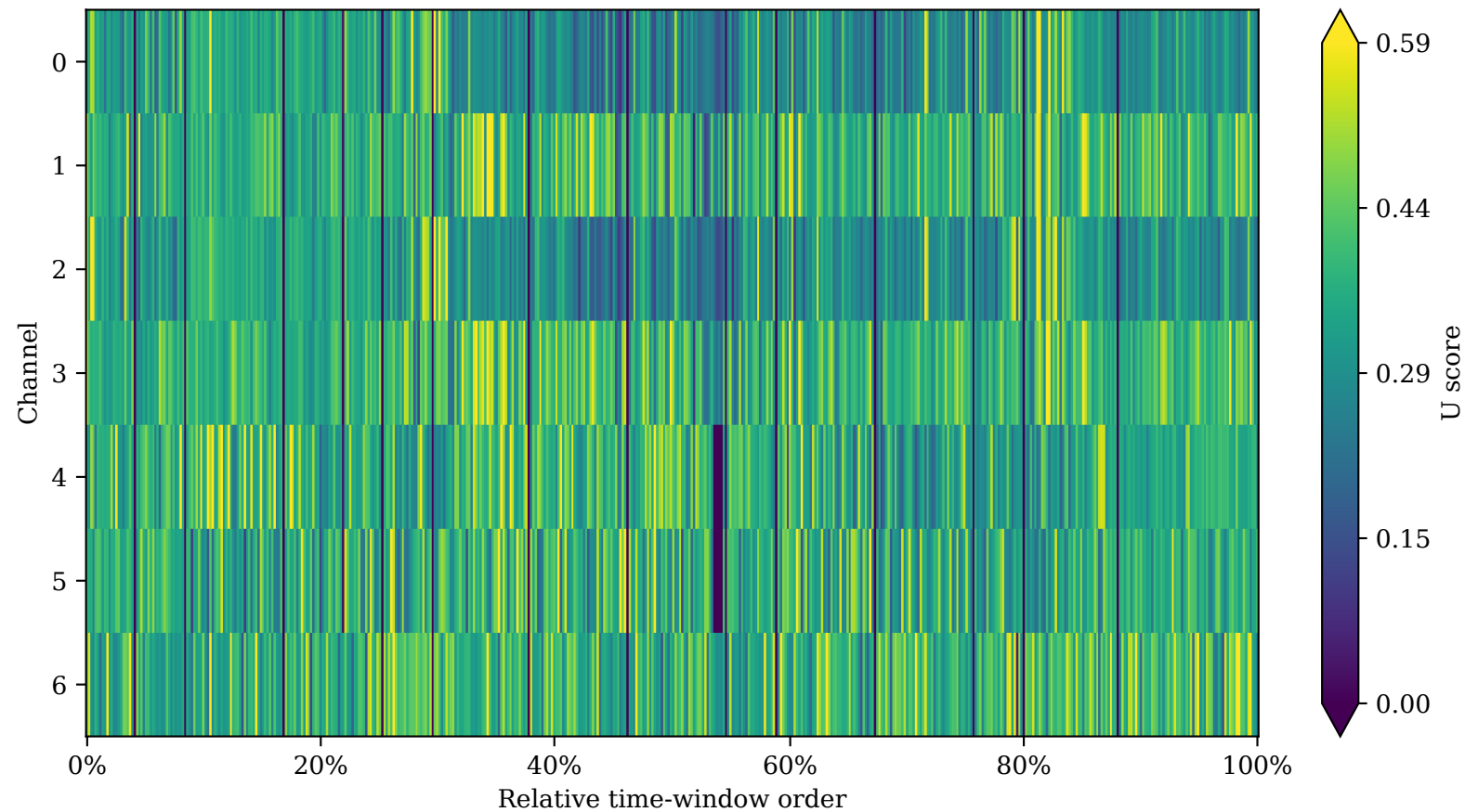
ETTm1: U across channels and time windows
