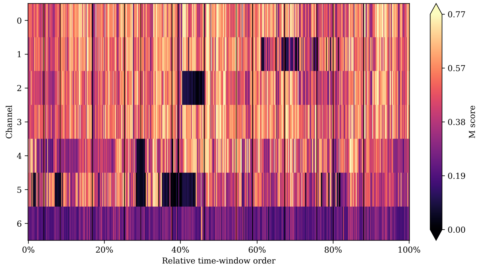
ETTm2: M across channels and time windows
