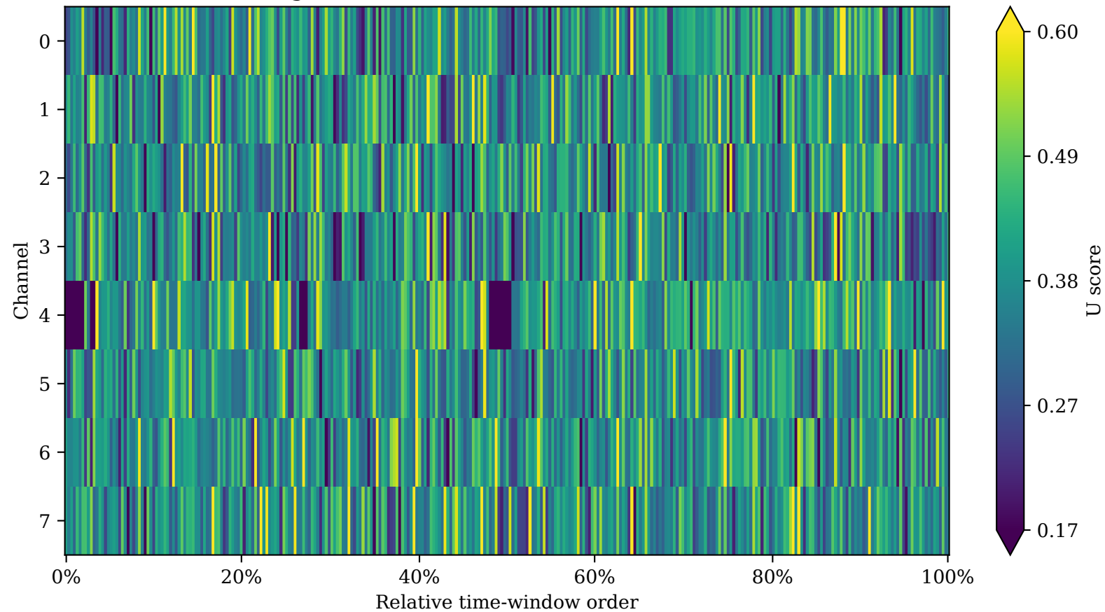
ExchangeRate: U across channels and time windows
