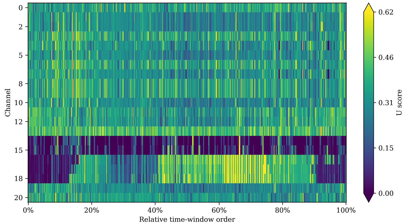
Weather: U across channels and time windows
