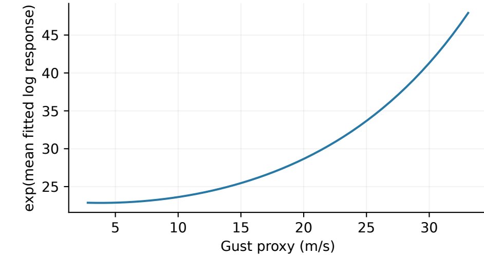
weather E0; n=9,857
