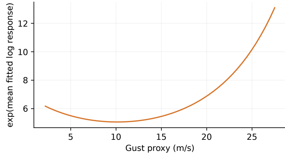
weather R0c; n=9,857
