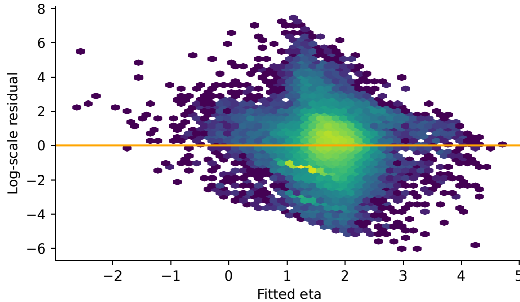
R0c residuals
