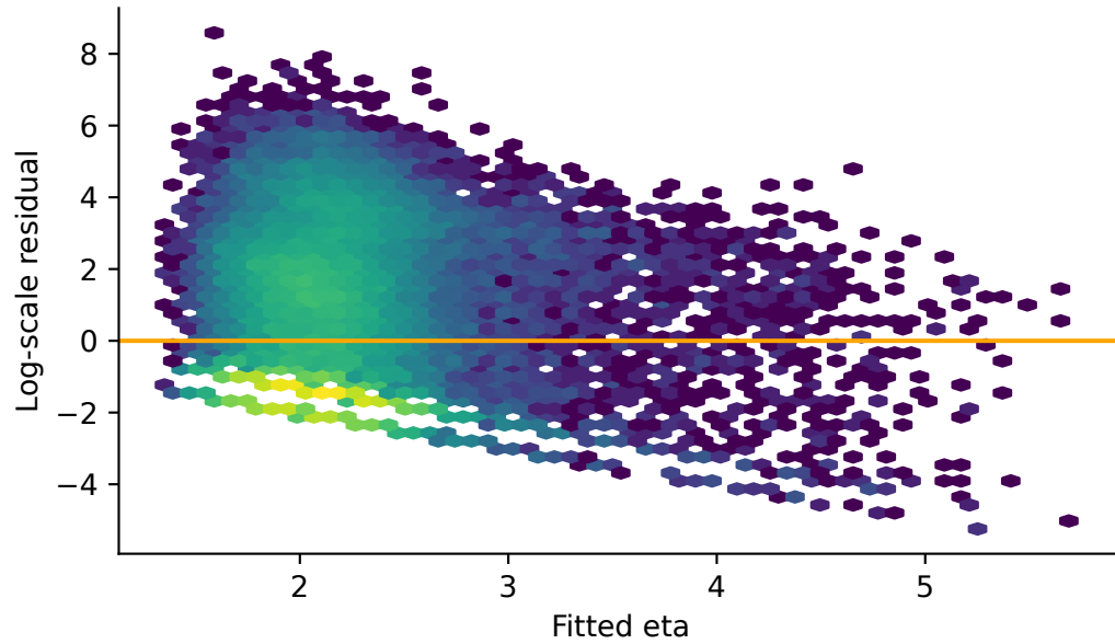
R0c residuals
