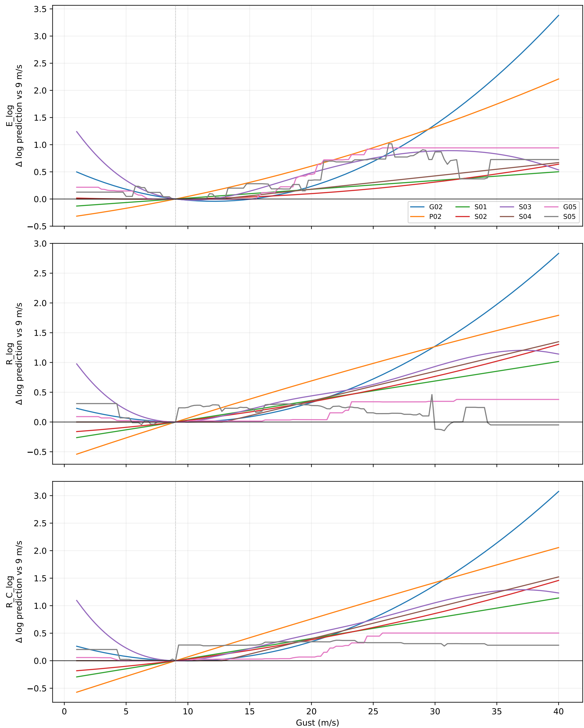
Frozen time-path gust response summaries (tree lines are average response, not structural laws)
