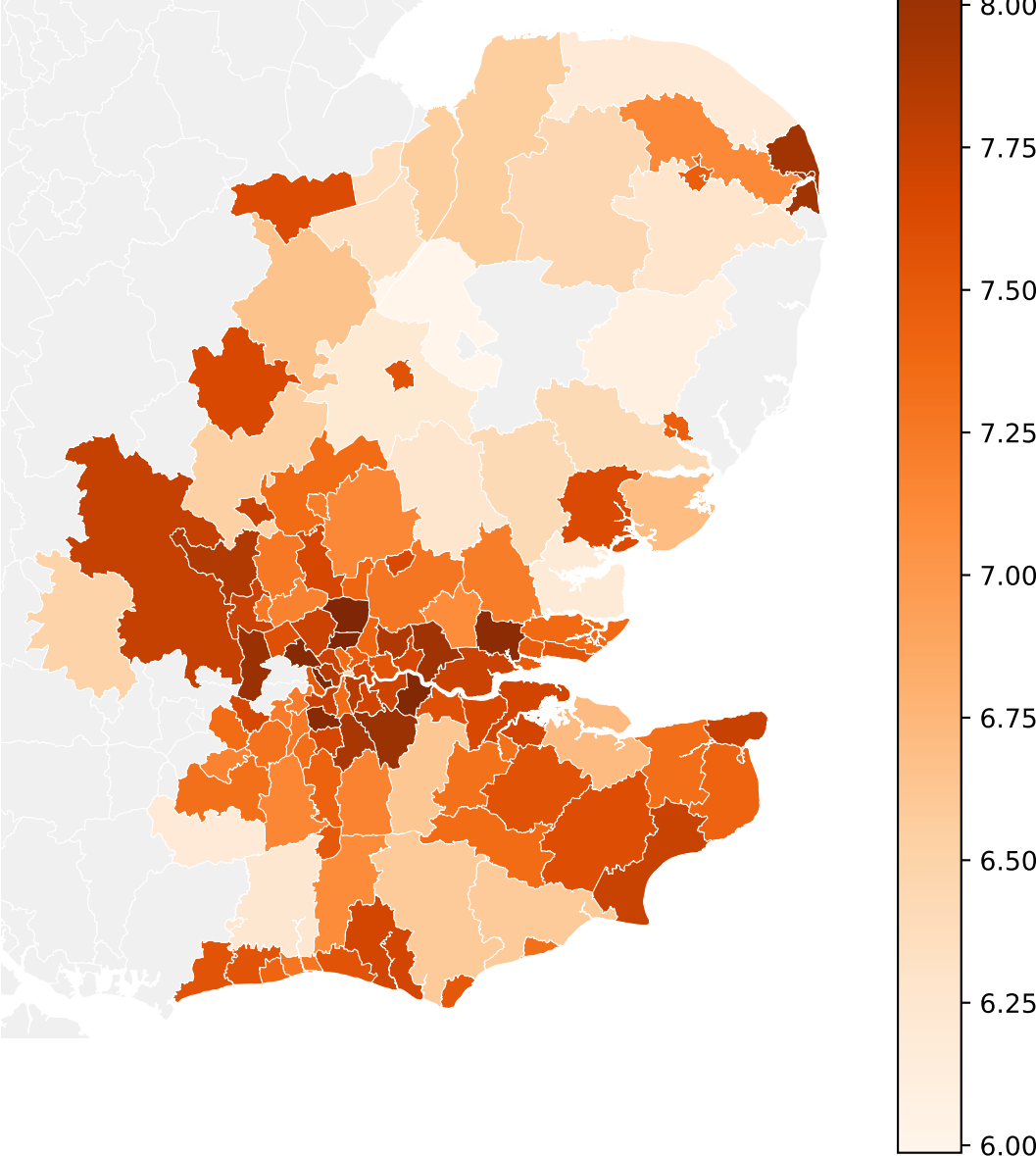
Baseline regional difference in predicted duration_B (fixed reference weather and customers_v2; region covariates vary)
