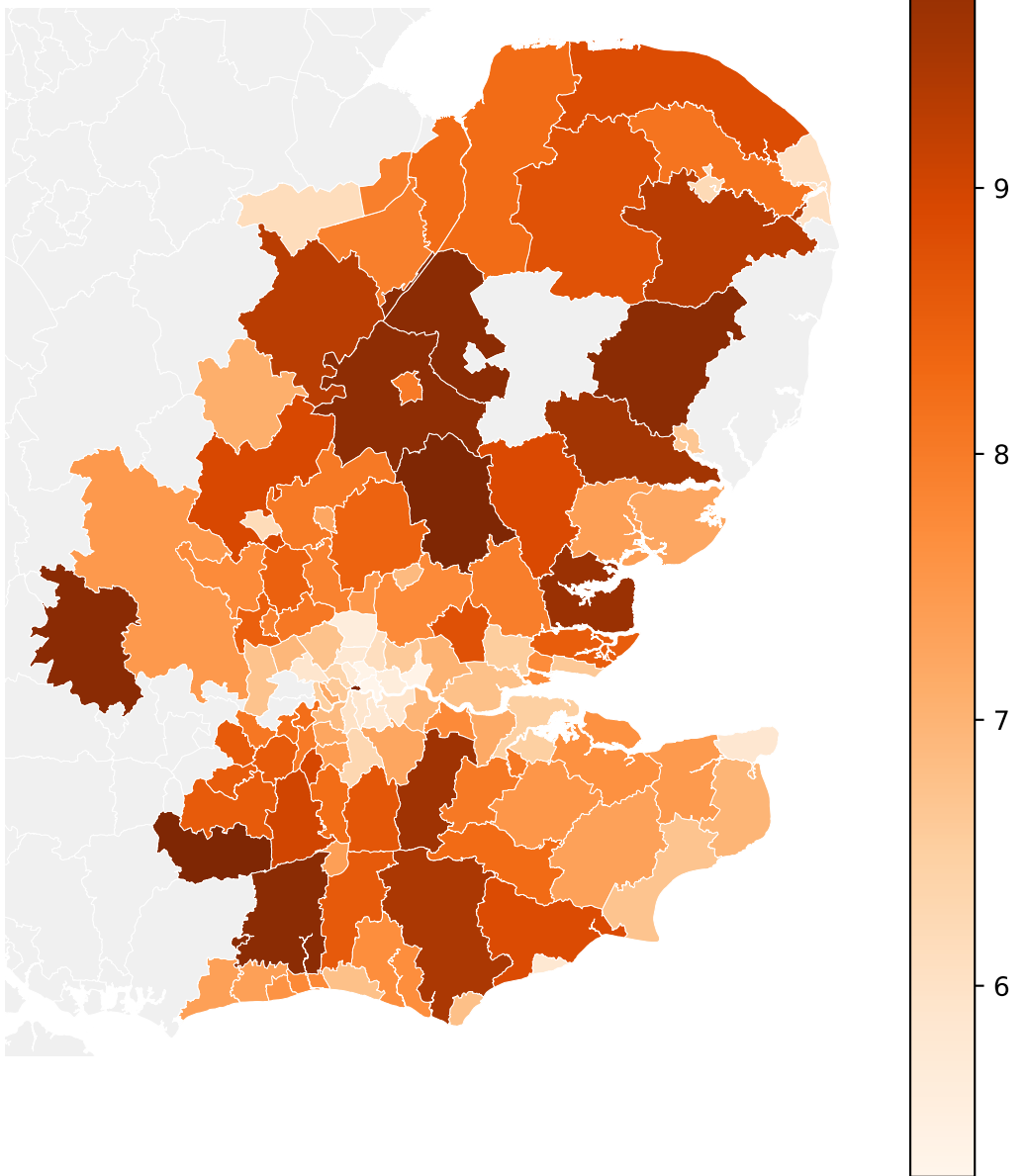
Baseline regional difference in predicted customers_v2 (fixed reference weather; region covariates vary)
