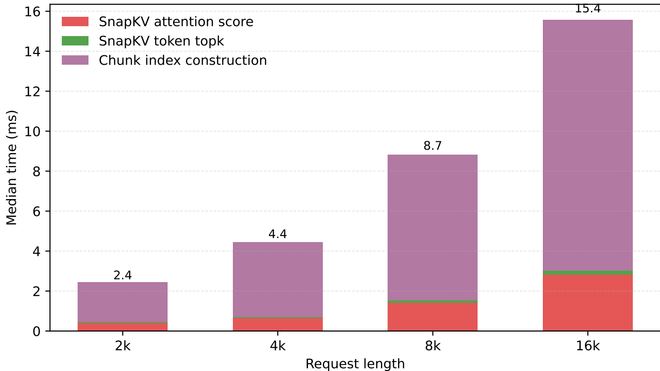
ChunkKV score/index overhead breakdown
