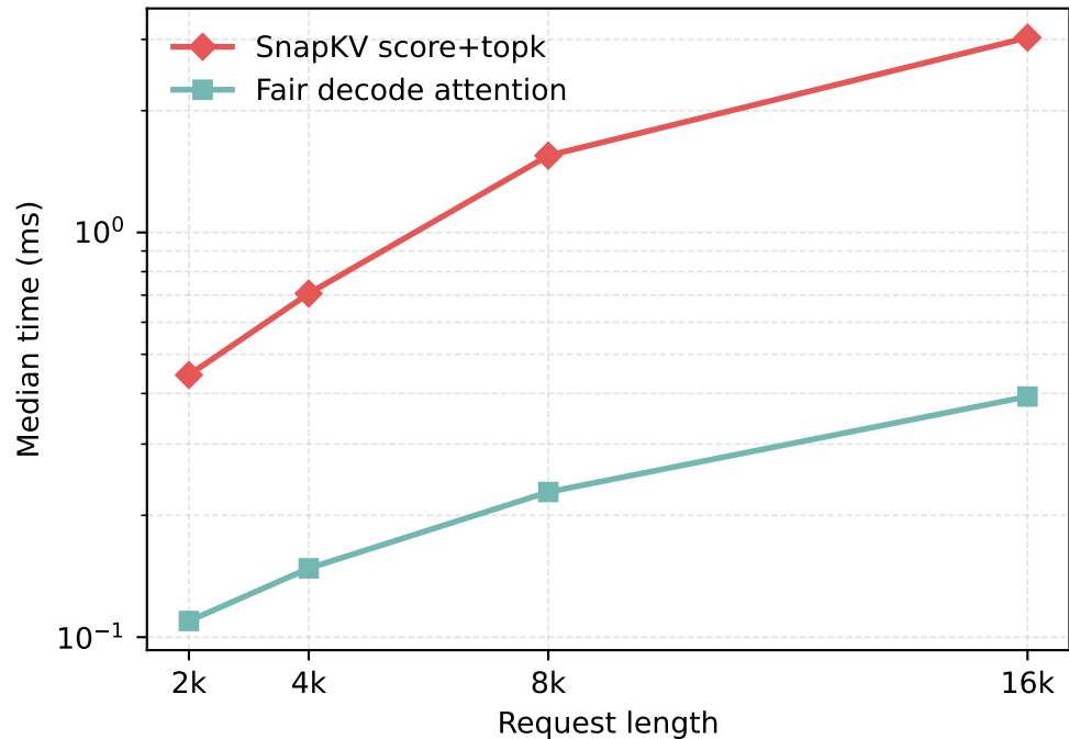
SnapKV index cost vs fair decode attention
