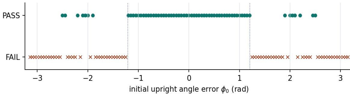
Figure 1. Signed offset sweep for pure LQR. Dotted lines mark the first near-upright pass/fail transition; they are not a global stability boundary.
