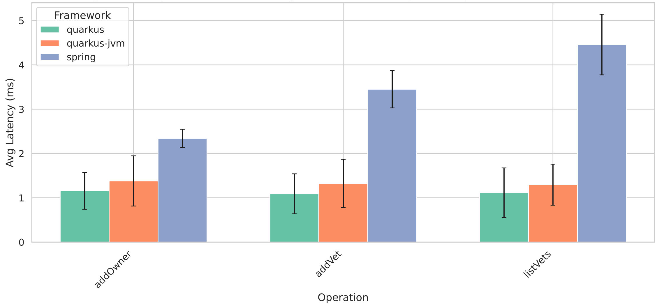
Figure 9: Per-Operation Framework Comparison (slsbench, lifecycle, steady, error bars = 1 std, n=6)
