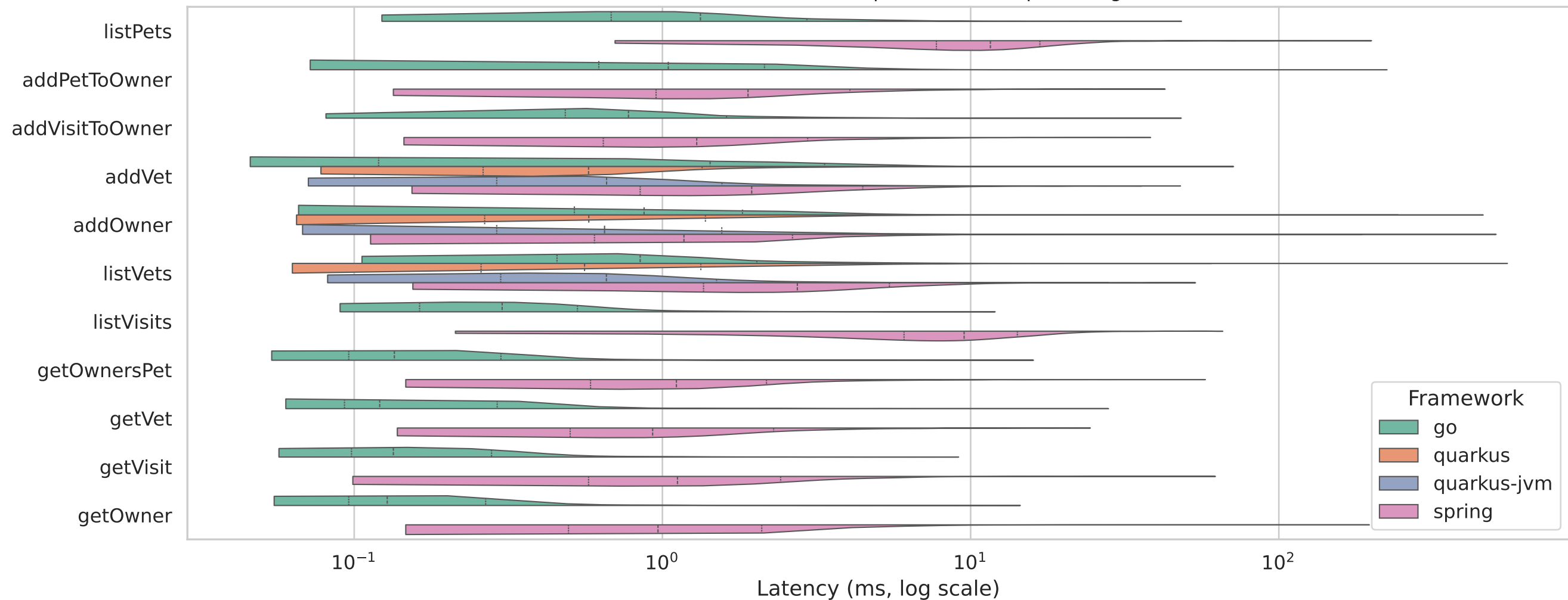
Figure 1: Per-Operation Latency Distributions (lifecycle, steady)
