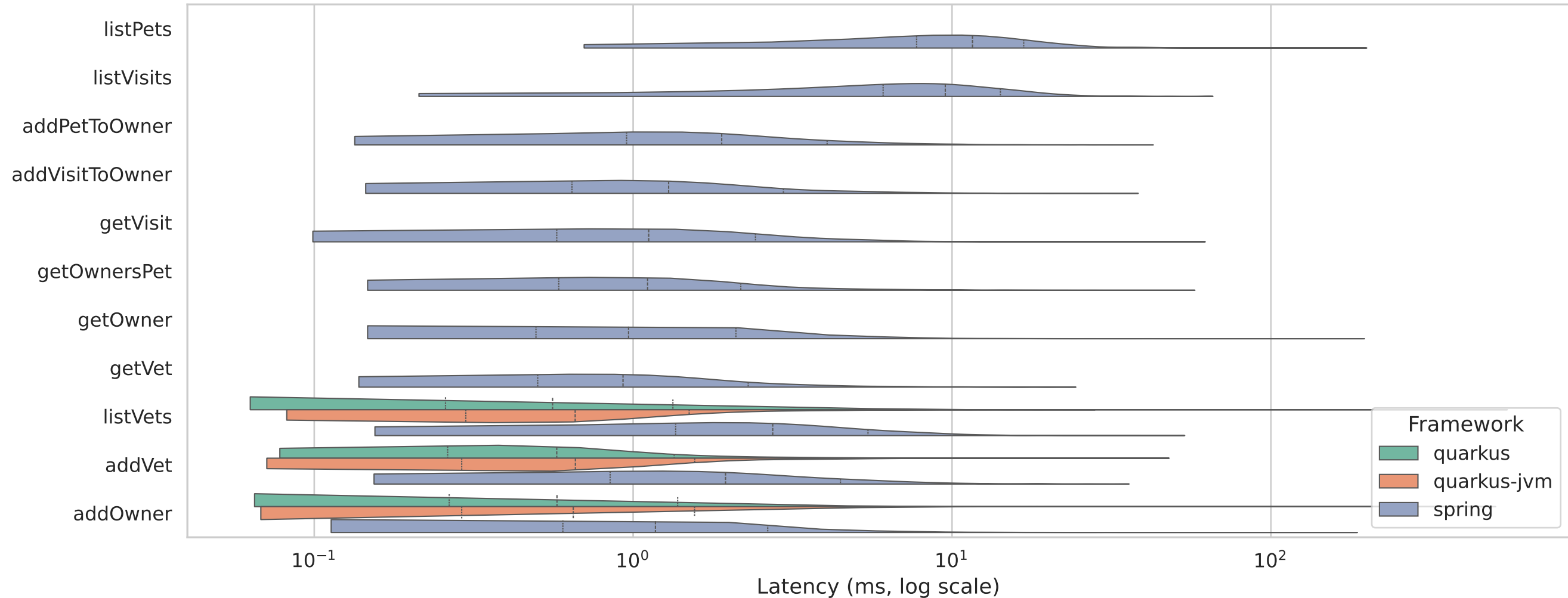
Figure 1: Per-Operation Latency Distributions (lifecycle, steady) n=115,970 individual requests, n=1 run per config
