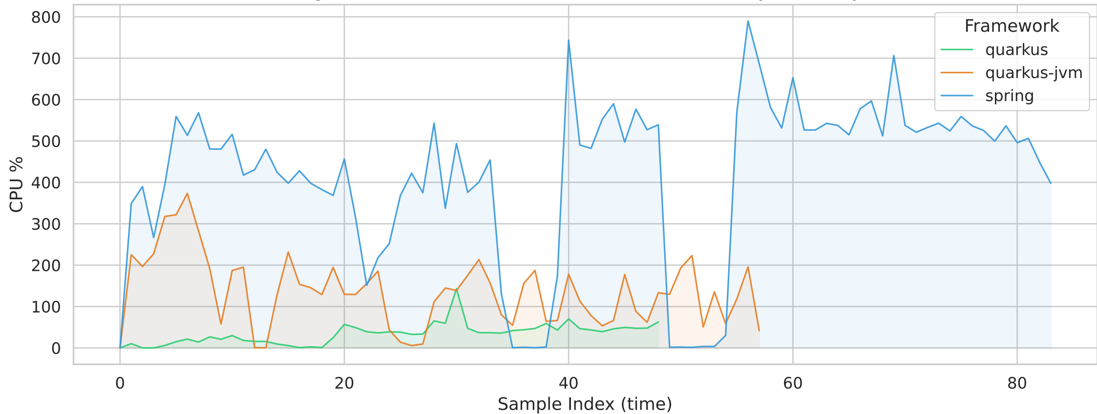
Figure 10: CPU Utilization Time-Series (slsbench, lifecycle, steady)
