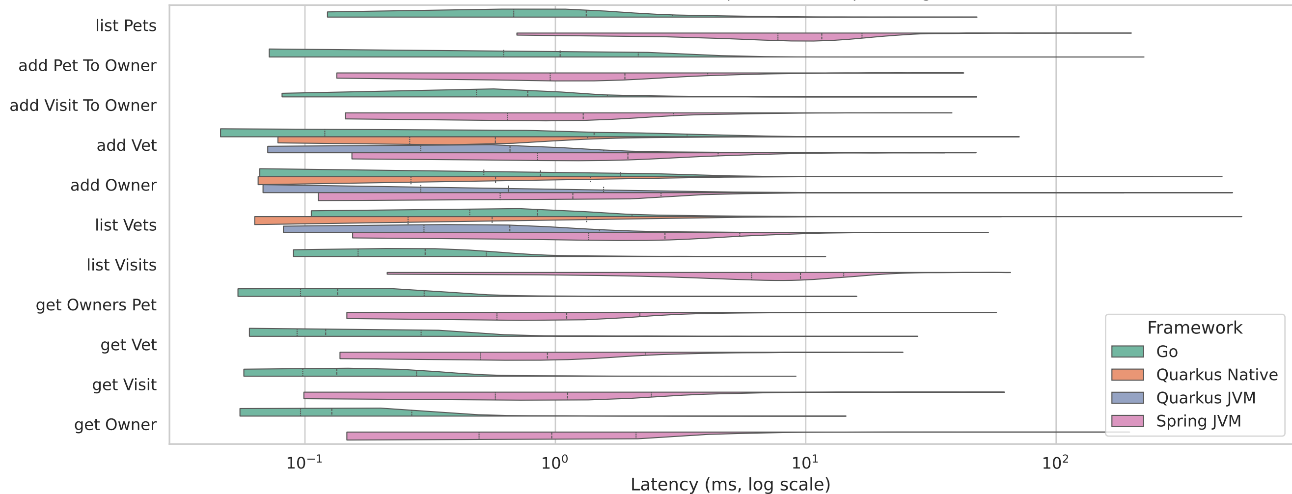
Figure 1: Per-Operation Latency Distributions (lifecycle, steady) n=189,260 individual requests, n=1 run per config
