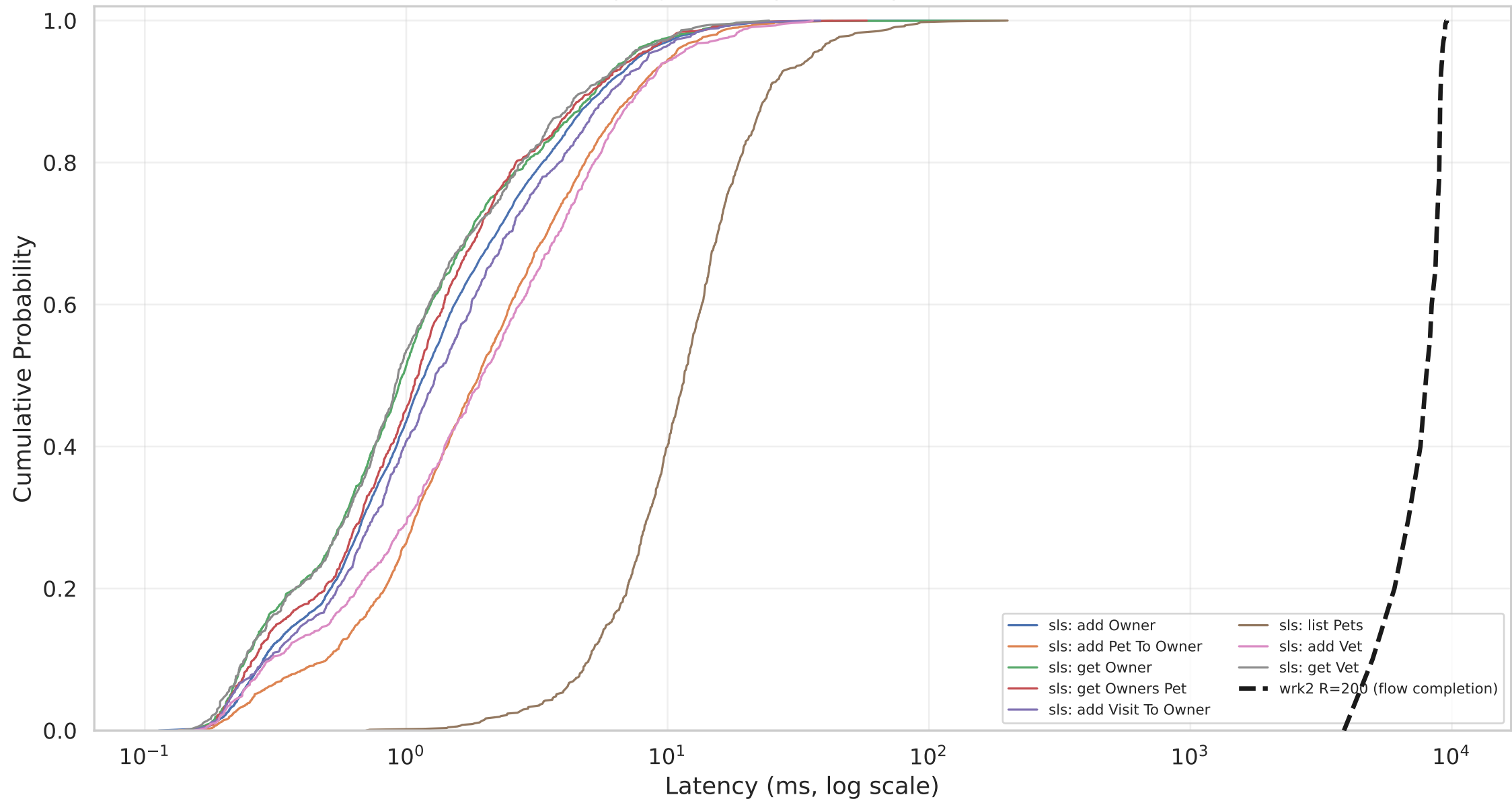
Figure 2: Latency CDF -- Per-Operation (slsbench) vs Aggregate (wrk2) Spring JVM, lifecycle, steady, n=1 run
