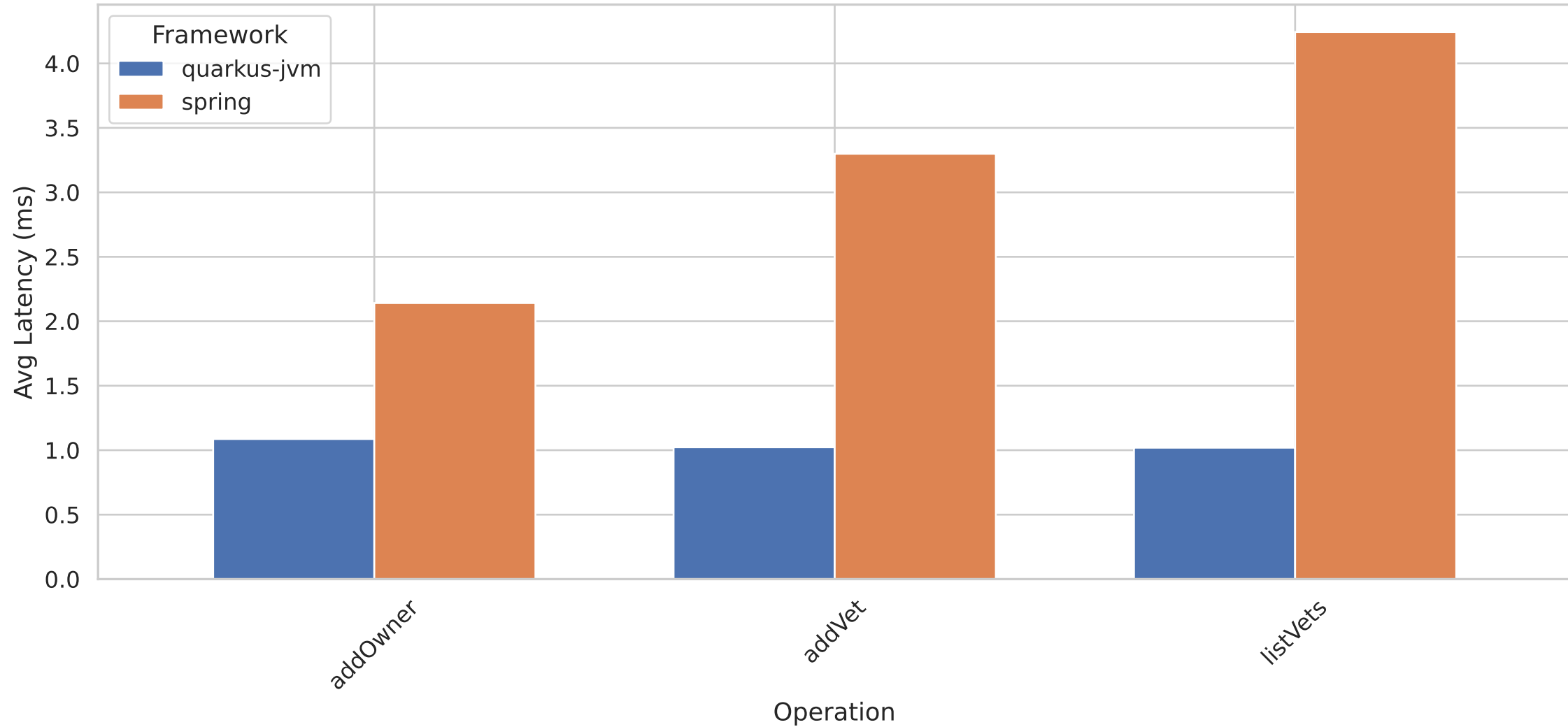
Chart D3: Per-Operation Framework Comparison (slsbench, lifecycle, steady)
