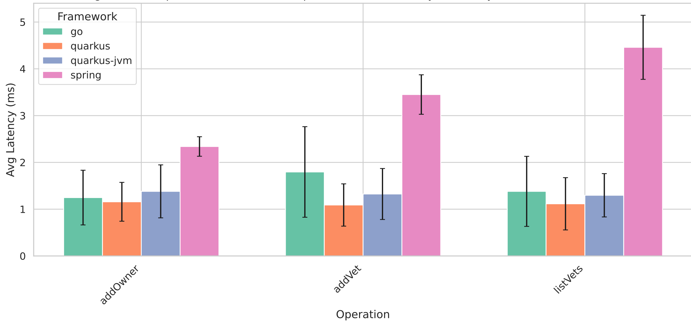
Figure 9: Per-Operation Framework Comparison (slsbench, lifecycle, steady, error bars = 1 std, n=12)
