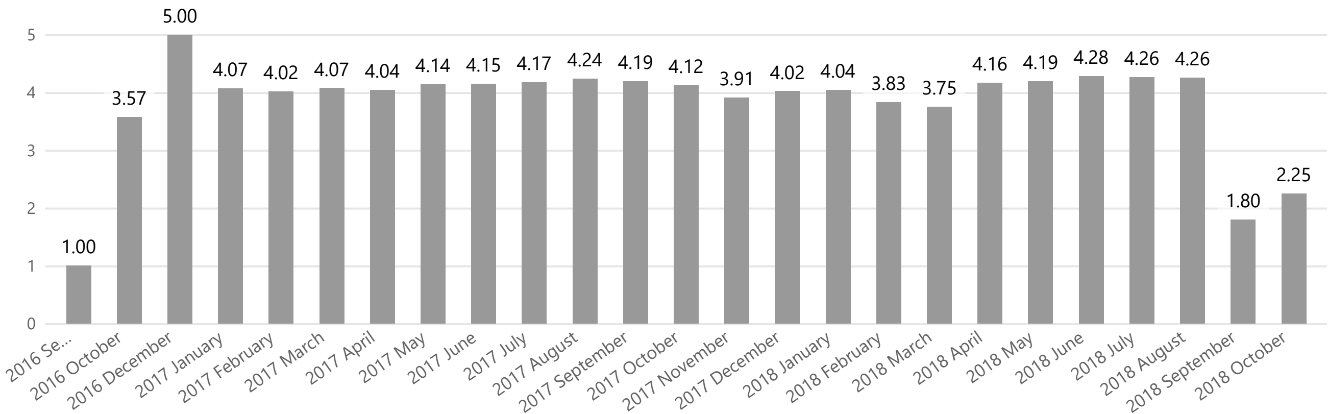
Stage_Total_Orders , Turnover_Rate
