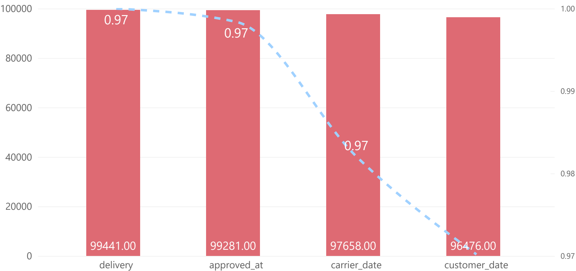
Stage_Total_Orders , Turnover_Rate
