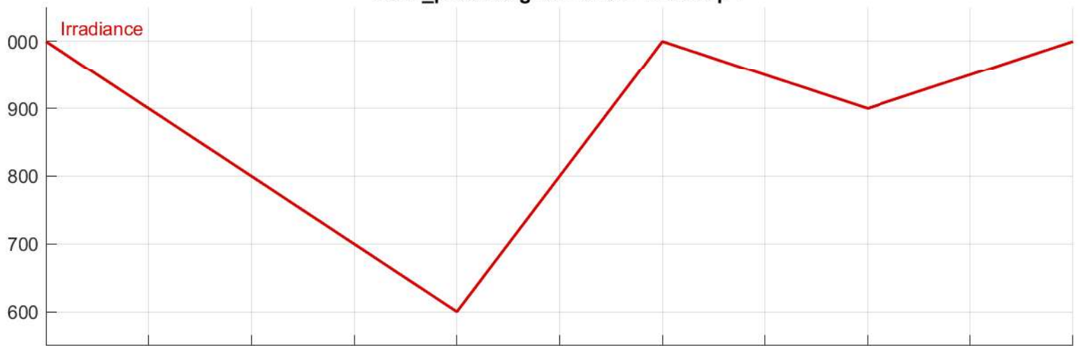
solar_pvadd/Signal Builder1 : Group 1
