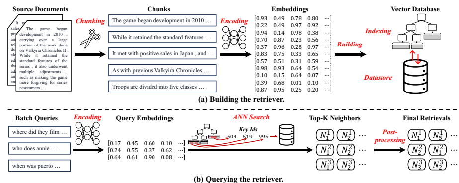
Fig. 2 Two stages of using the retriever
