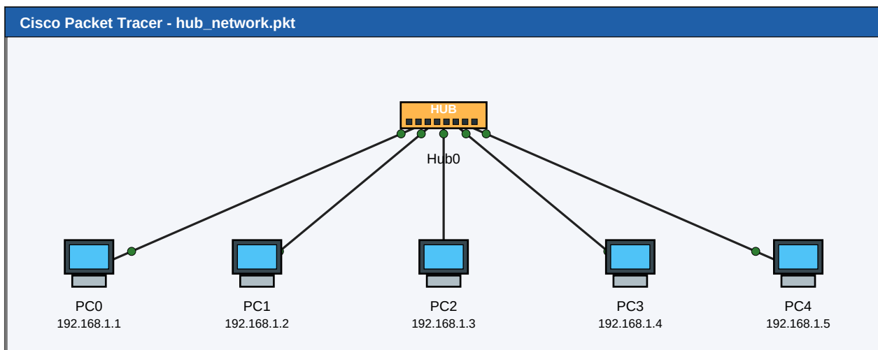
Experiment 1 : hub network in Packet Tracer (all link lights green)
