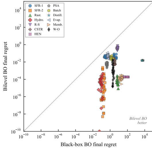
Figure 7: Scatter plot of final regret: black-box BO vs. bilevel BO. Each point is one (problem, n_{\text{init}} , \xi ) configuration. All points lie below the diagonal.
