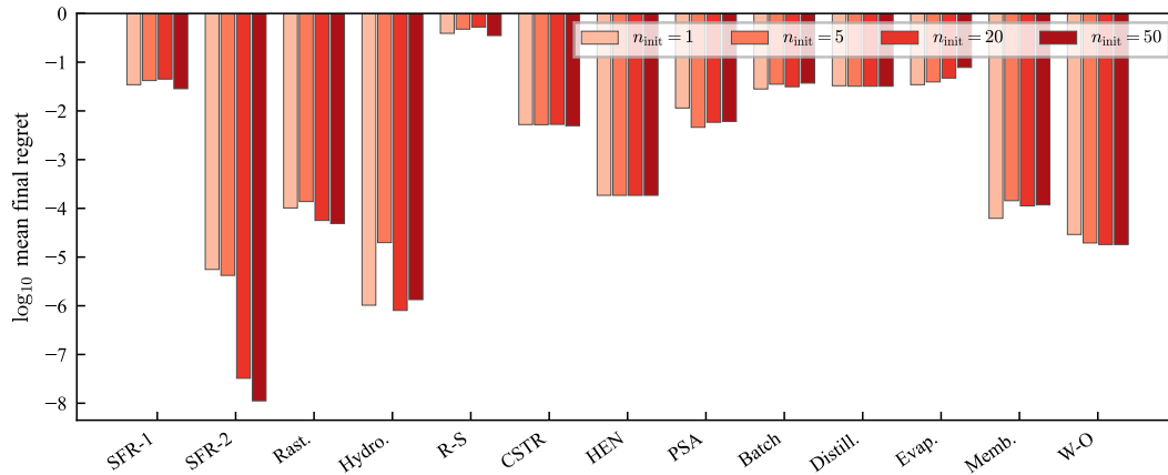
Figure 8: Sensitivity to n_{\text{init}} . Final regret ( \log_{10} scale) of bilevel BO is nearly flat across n_{\text{init}} \in \{1, 5, 20, 50\} , using the best \xi per problem. Even n_{\text{init}} = 1 performs comparably to n_{\text{init}} = 50 , indicating that fewer expensive initial evaluations suffice.
