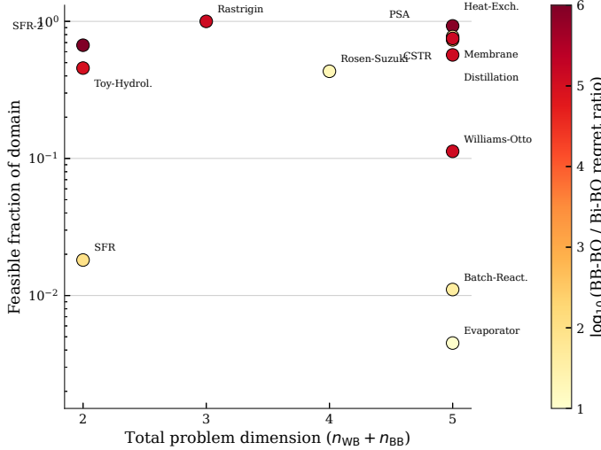
Figure 10: Regret ratio decomposed by total dimension and constraint tightness. Each point is one benchmark problem; color encodes \log_{10}(\text{BB-BO} / \text{Bi-BO regret ratio}) . The feasible fraction of the domain is estimated by 10^5 uniform random samples. Dimensionality reduction is the dominant factor; constraint tightness modulates but does not determine the advantage.
