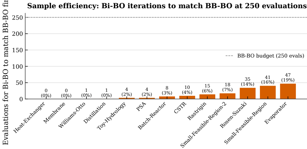
Figure 11: Sample efficiency crossover: number of evaluations for bilevel BO to match black-box BO’s final regret (at 250 evaluations). Percentages show the fraction of the total budget required. On 10 of 13 problems, bilevel BO matches black-box BO’s final performance within 10% of the evaluation budget.
