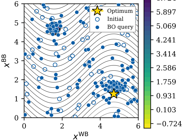
Black-box BO
