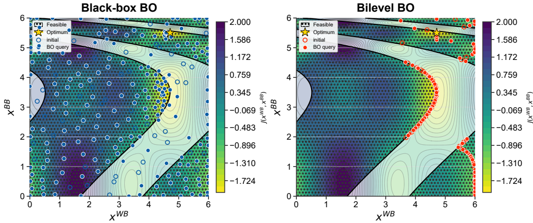
SFR-2: Final state (50 initial + 200 BO iterations)
