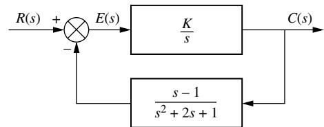
FIGURE P6.9
