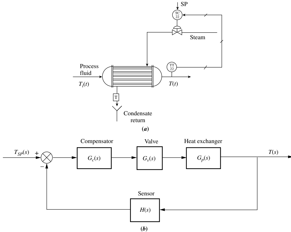
FIGURE P9.6 a. Heat-exchanger process (Reprinted with permission of John Wiley & Sons, Inc.); b. block diagram
