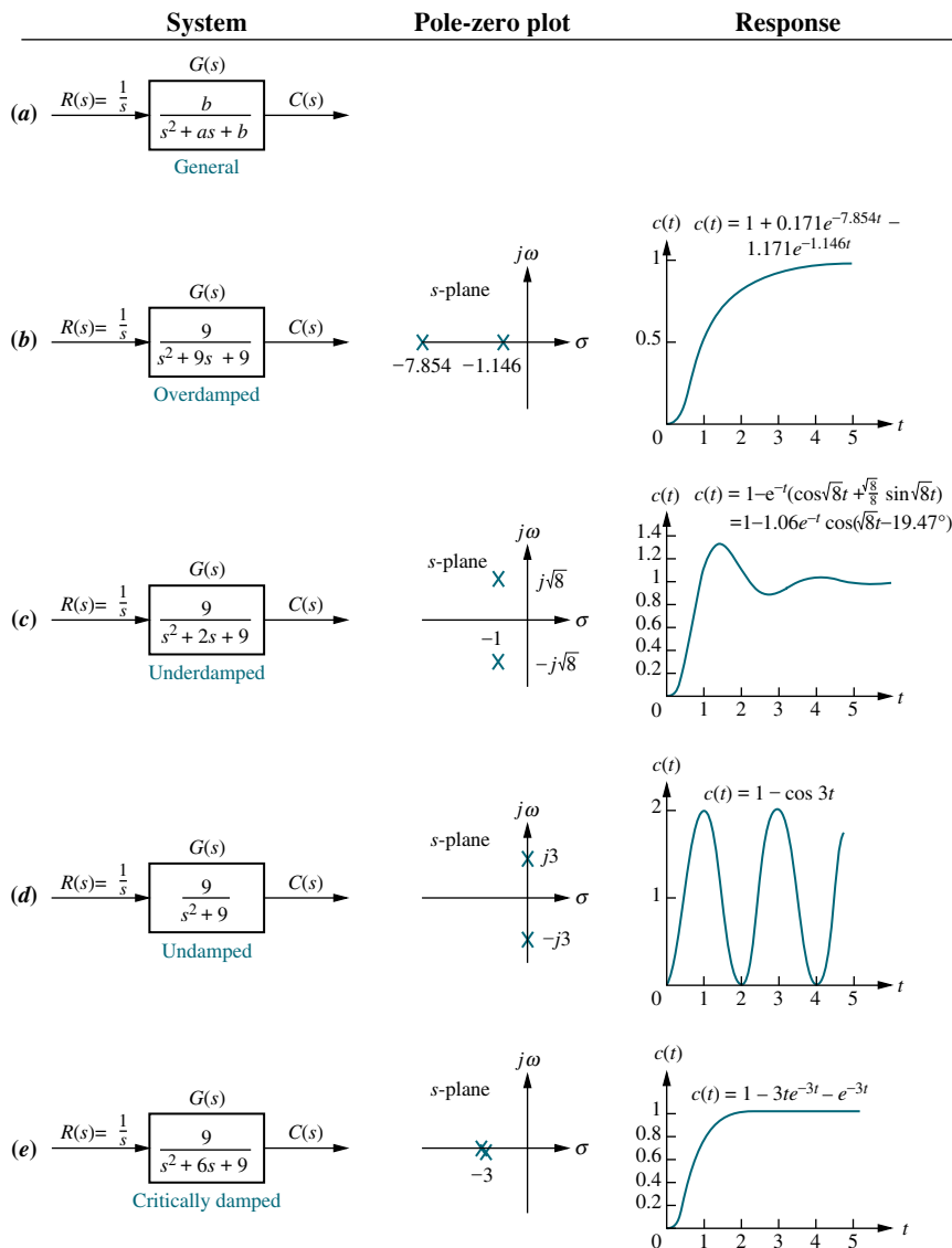
FIGURE 4.7 Second-order systems, pole plots, and step responses
