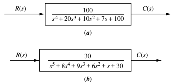
FIGURE P3.8
