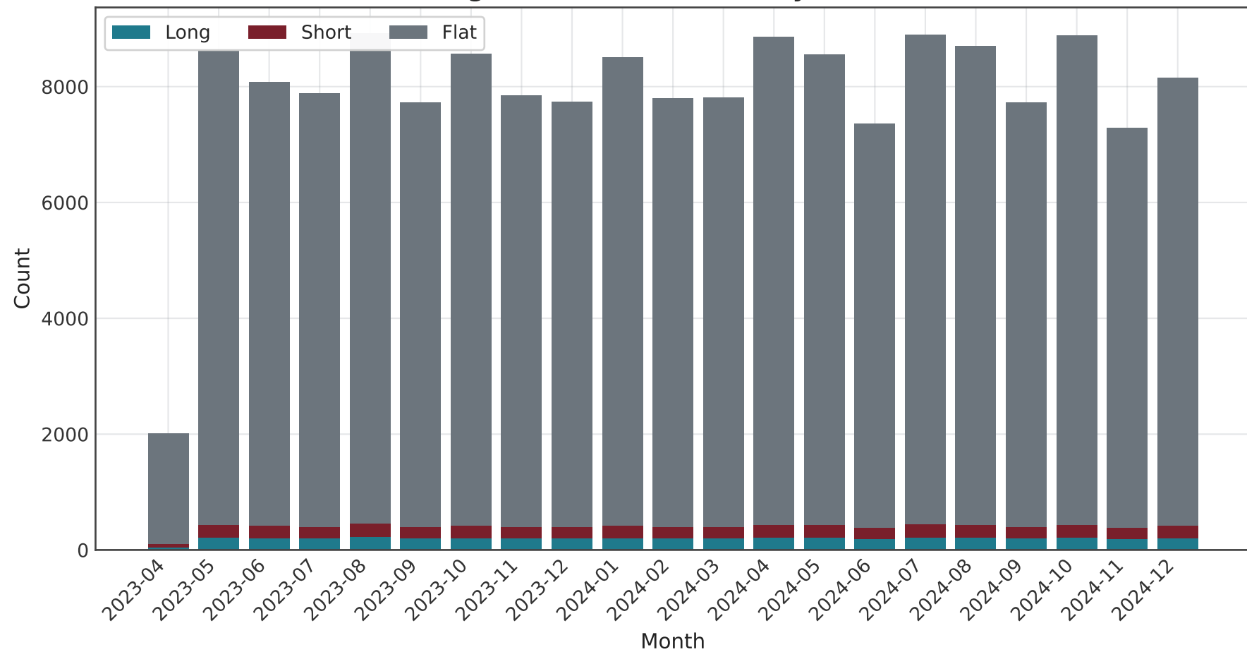
Signal Direction Counts by Month
