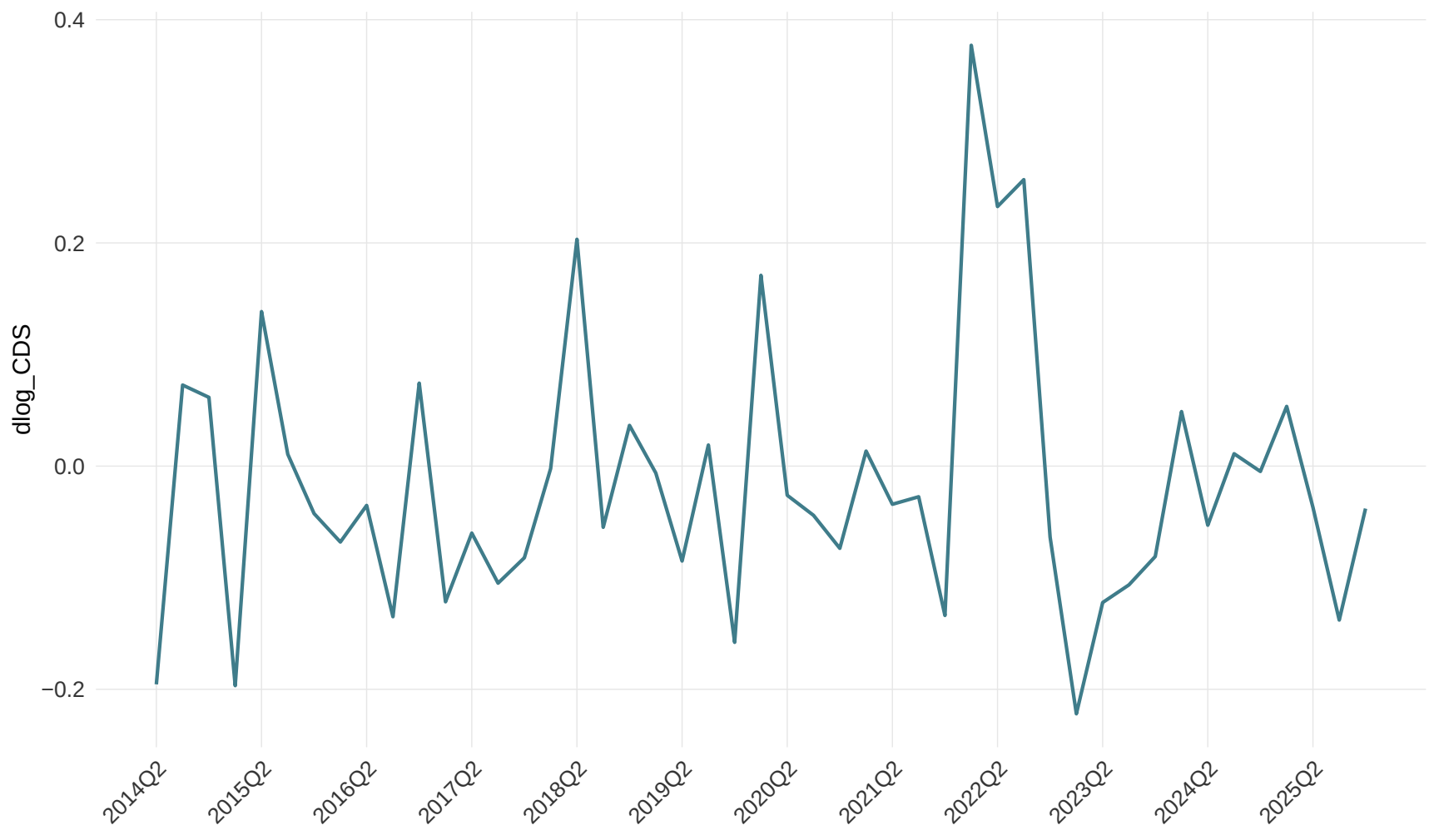
Panel-average time series: dlog_CDS
