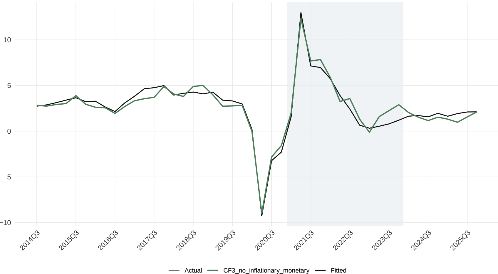
GDP_Growth counterfactual: CF3_no_inflationary_monetary Model-implied counterfactual path; shaded area marks 2021Q1–2023Q4.
