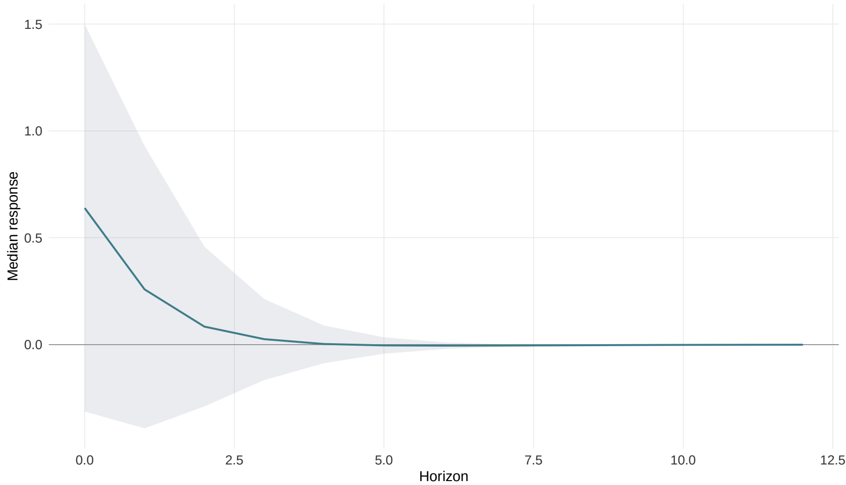
Sovereign-risk repricing shock -> GDP_Growth
