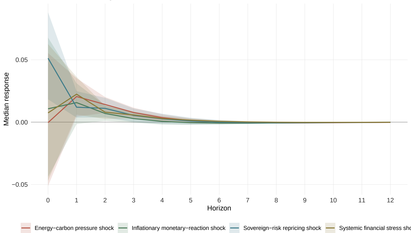
Structural IRFs of dlog_CDS to all identified shocks
