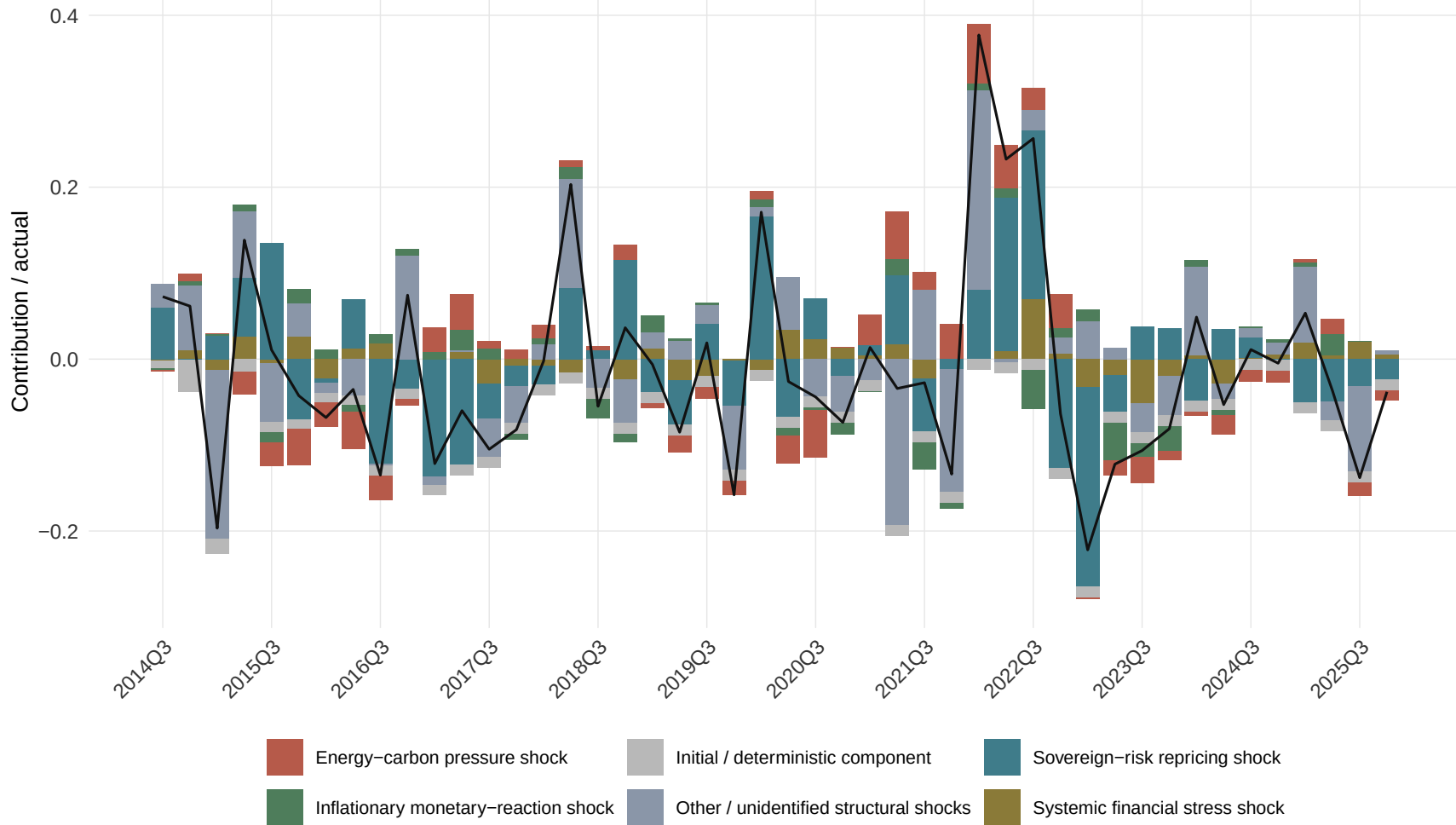
Panel-average HD: dlog_CDS
