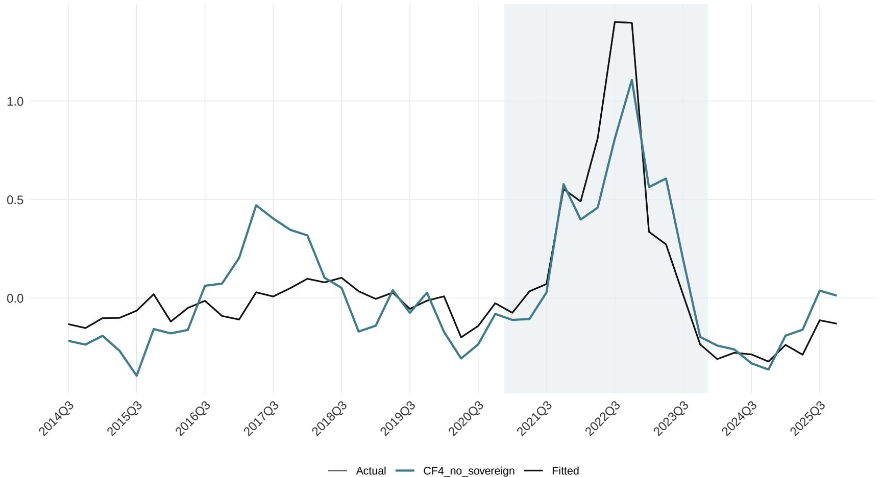
d_3MRate counterfactual: CF4_no_sovereign Model-implied counterfactual path; shaded area marks 2021Q1–2023Q4.
