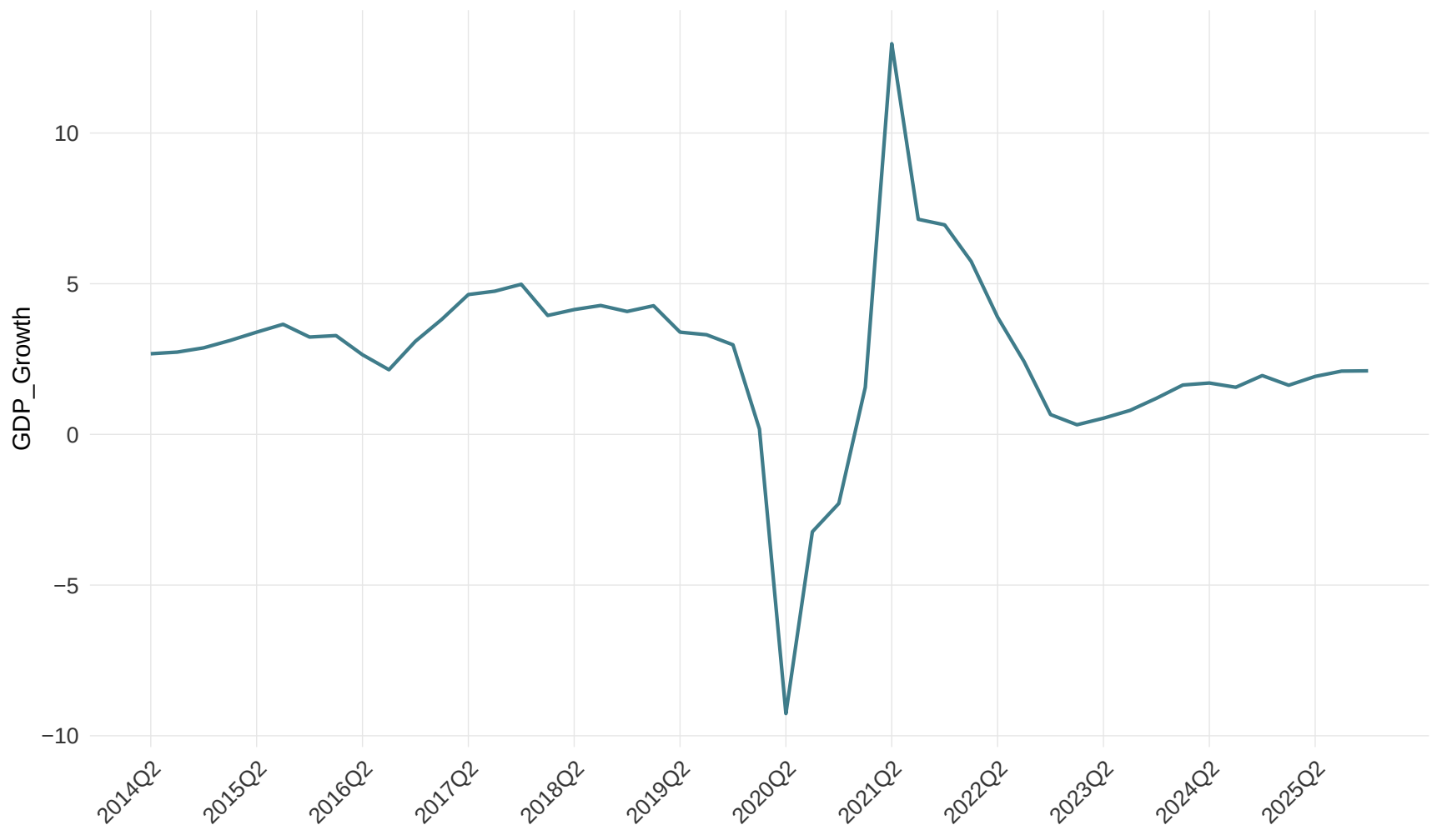
Panel-average time series: GDP_Growth
