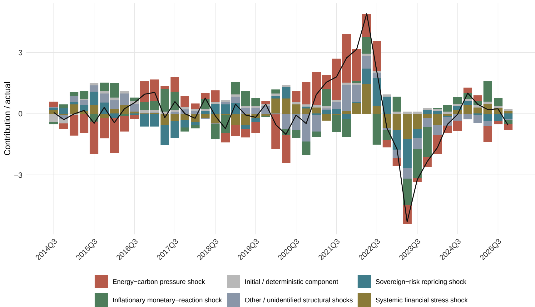
Panel-average HD: d_CPI
