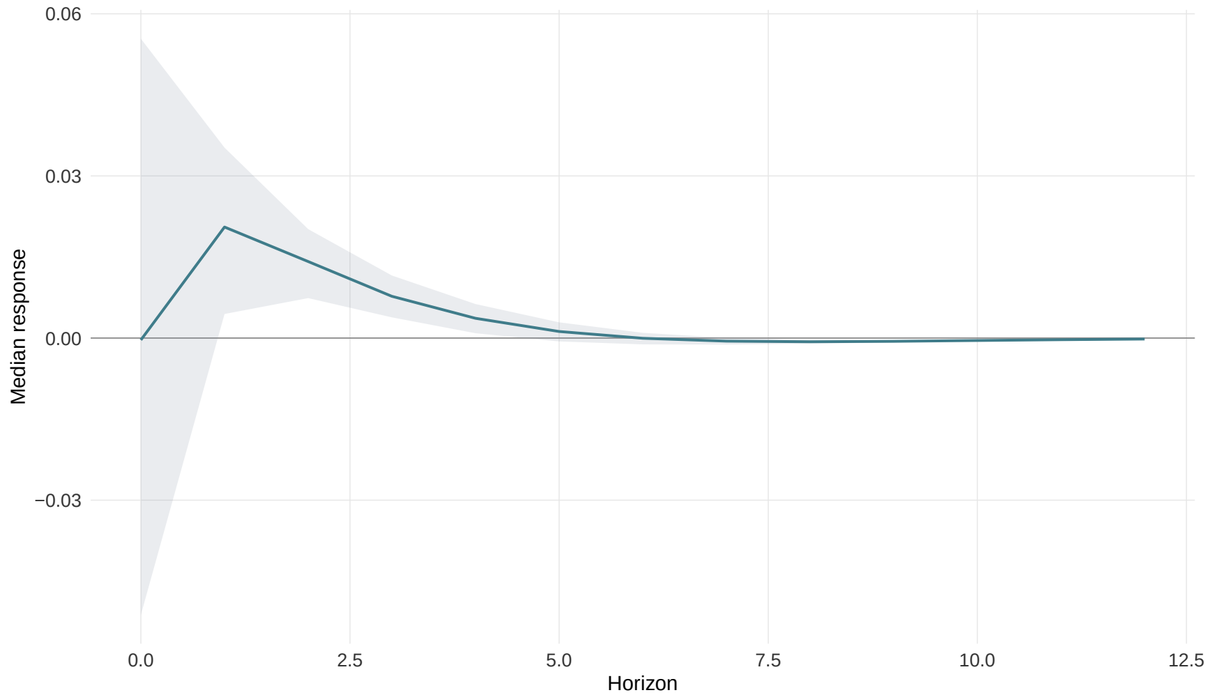
Energy-carbon pressure shock -> dlog_CDS
