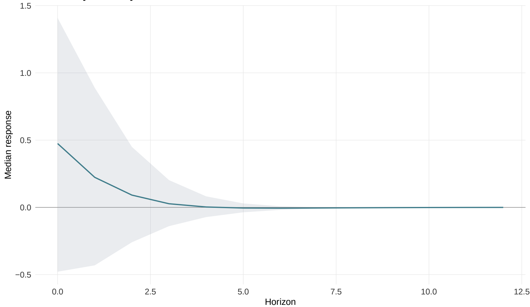
Inflationary monetary-reaction shock → GDP_Growth
