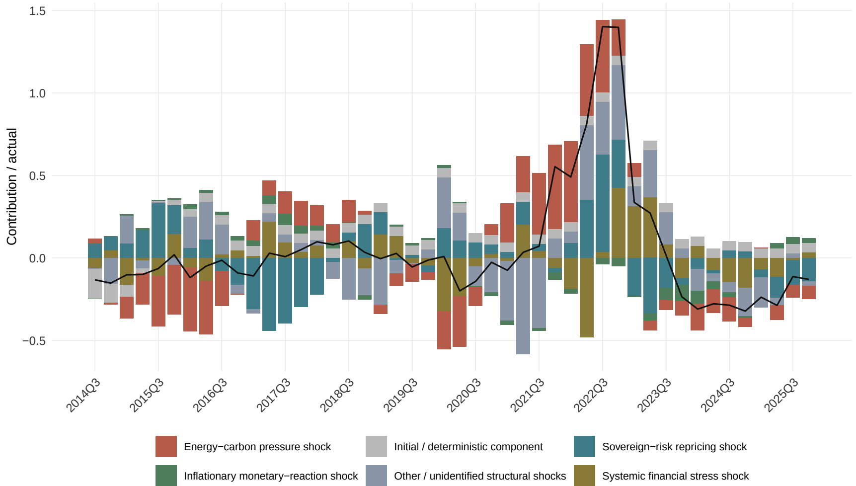
Historical decomposition of panel-average d_3MRate
