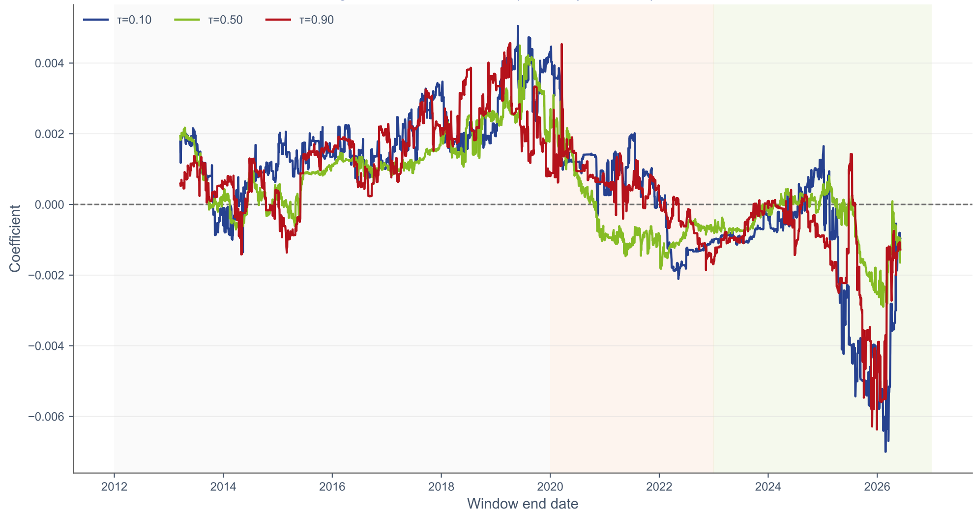
Rolling Quantile Coefficients (252-Day Window): \Delta\text{Bund } 10Y
