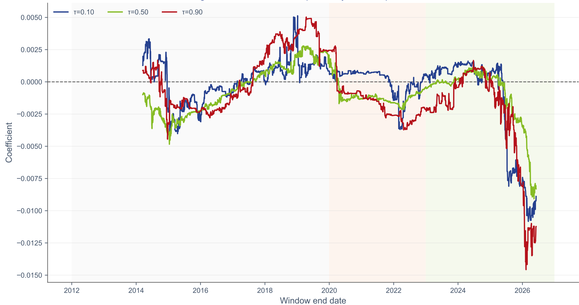
Rolling Quantile Coefficients (504-Day Window): Brent Return
