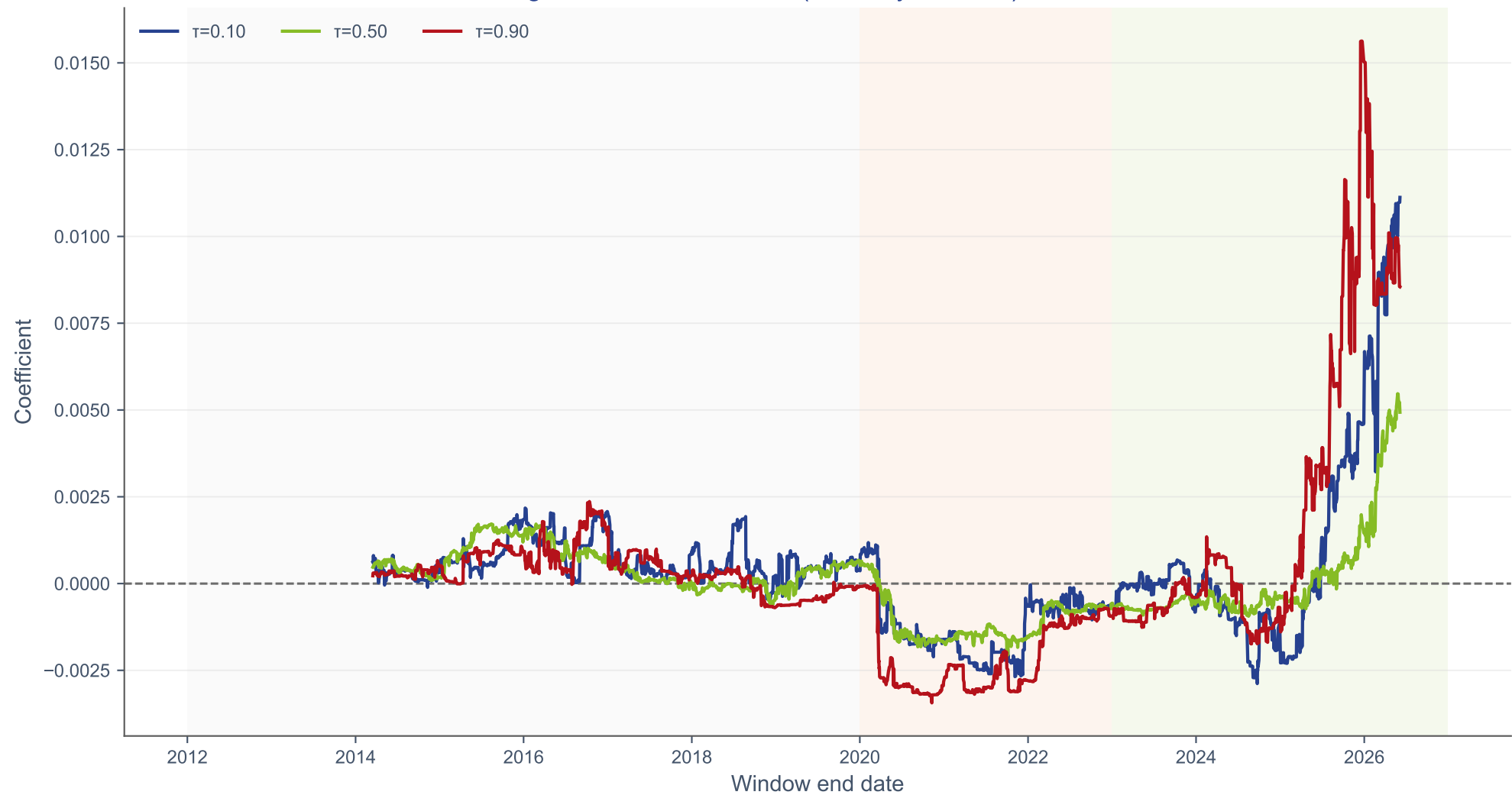
Rolling Quantile Coefficients (504-Day Window): EUA Return
