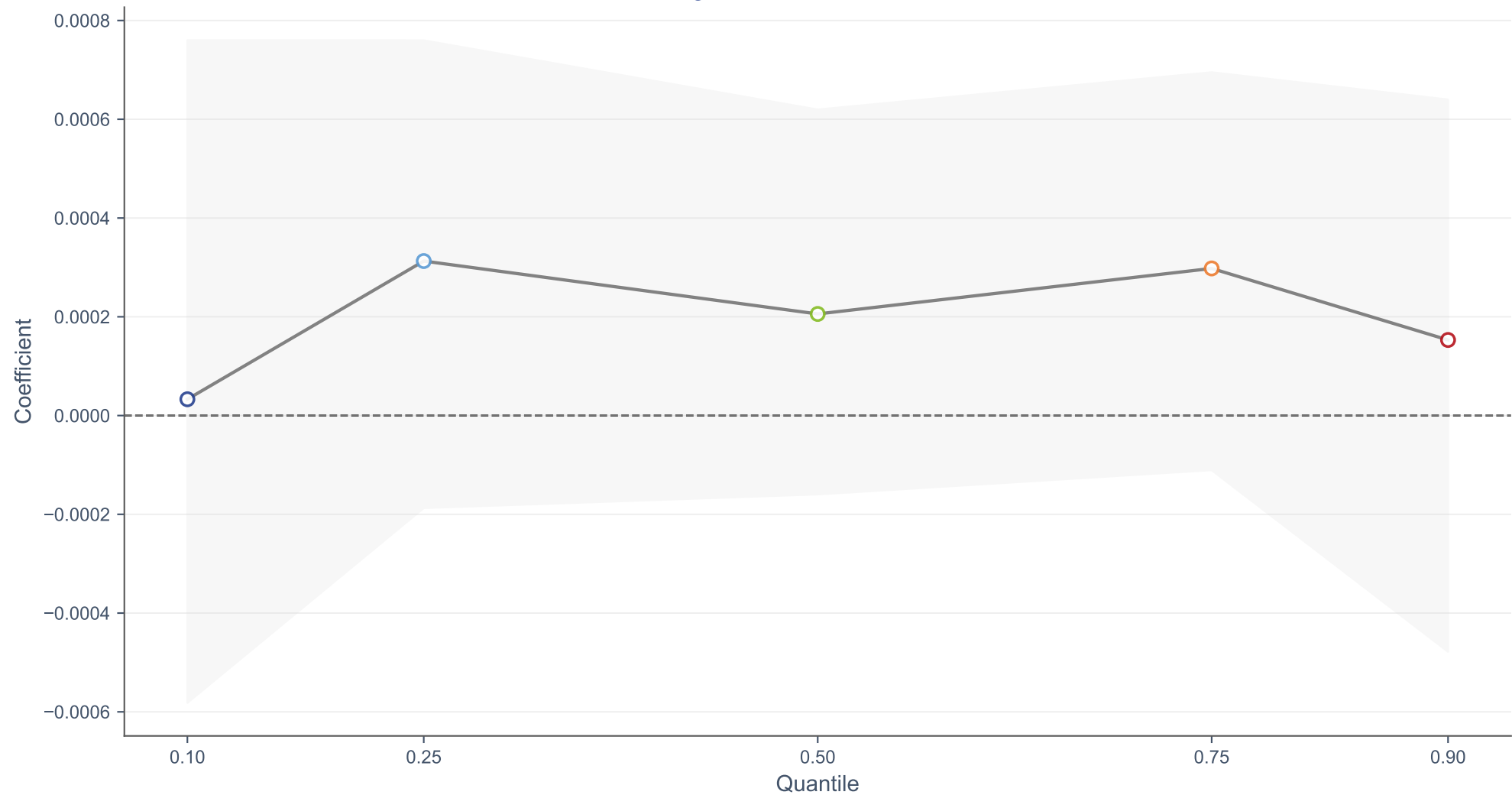
Quantile Regression Coefficients: \Delta\text{Bund 10Y}
