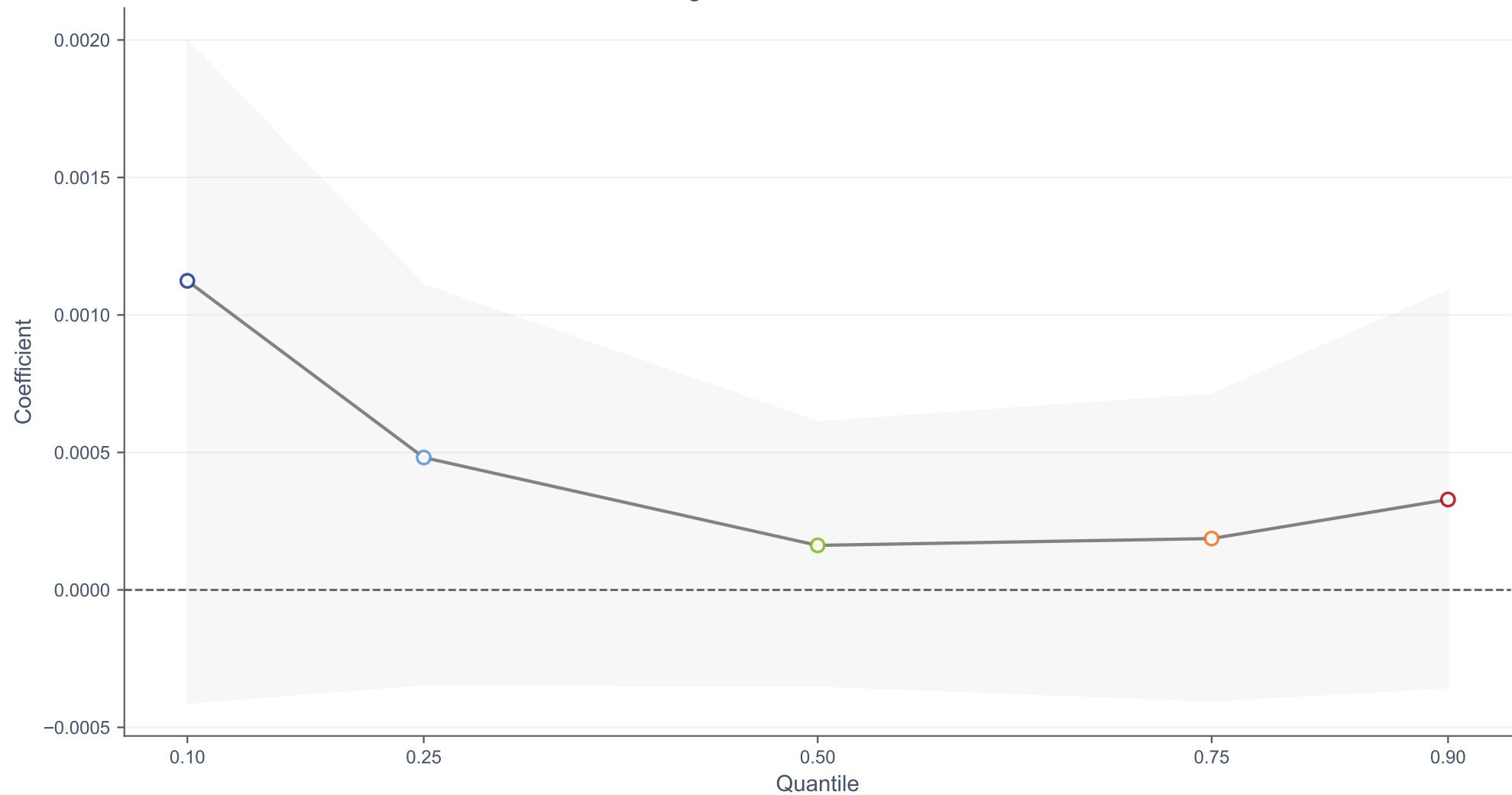
Quantile Regression Coefficients: EUA Return
