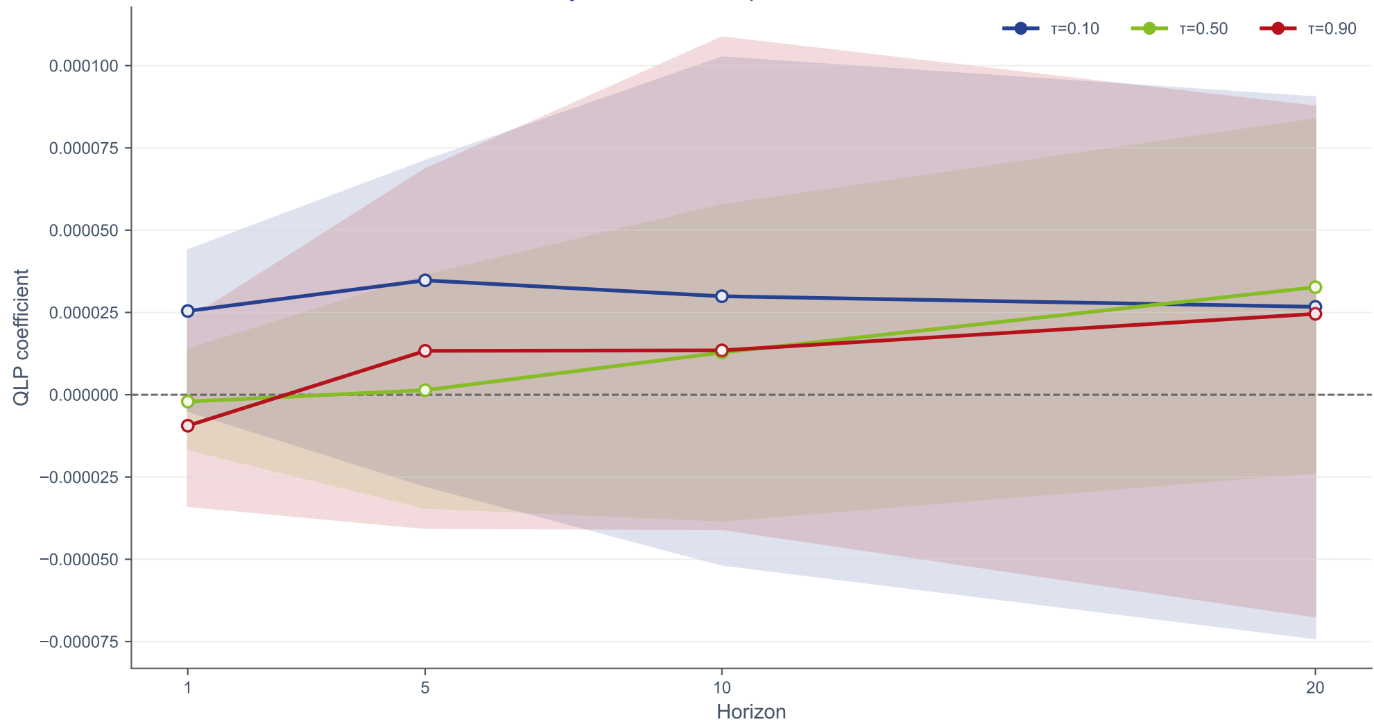
Dynamic QLP Responses: \Delta VSTOXX
