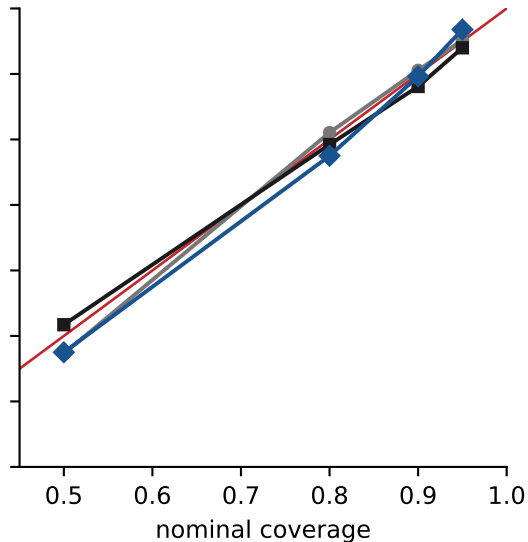
CQR (adaptive width)
