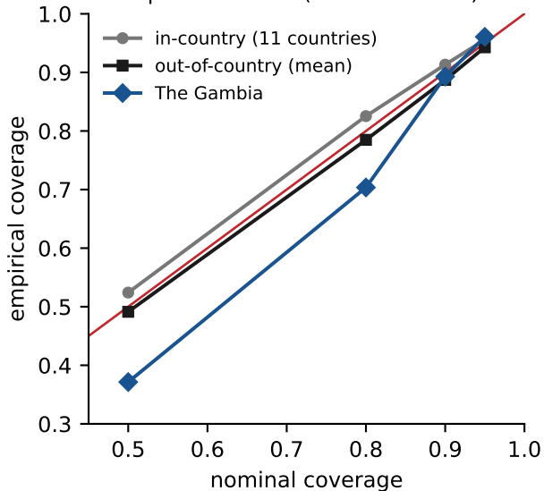
Split conformal (constant width)
