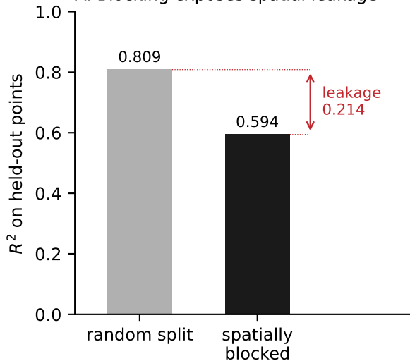
A. Blocking exposes spatial leakage
